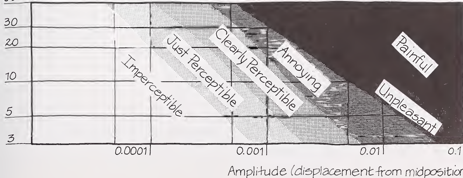
Human Sensitivity to Vibration (Reiher-Meister Scale) (Australian Study)
